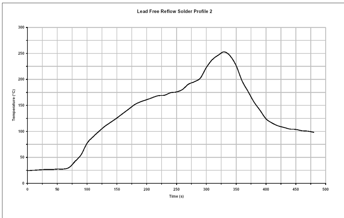
Figure 31: Reflow solder profile
