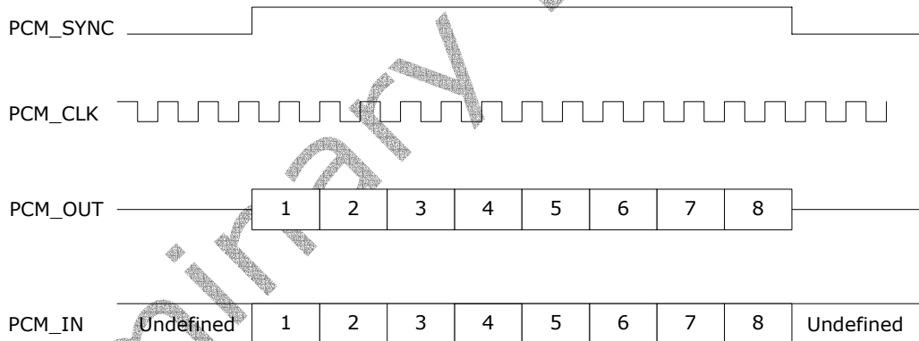
Figure 15: Long frame sync (shown with 8-bit Companded Sample)
