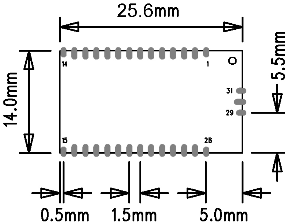
Figure 2: WRAP THOR WT12 foot print and dimension
