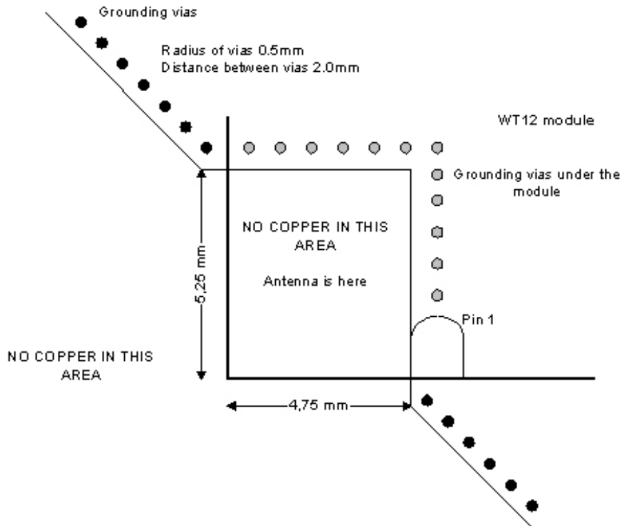
Figure 4: PCB design around ACX antenna
