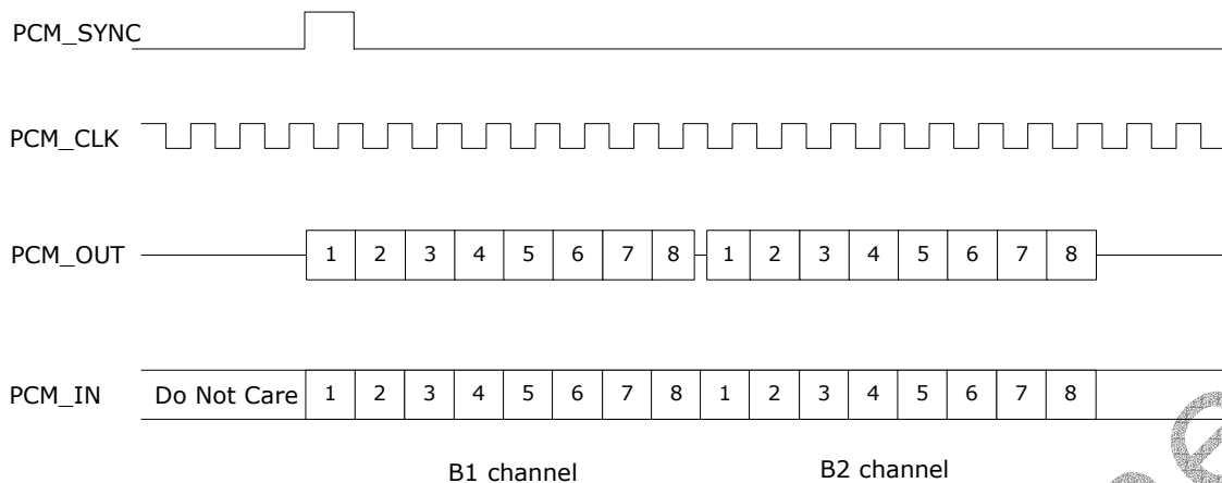
Figure 18: GCI Interface
