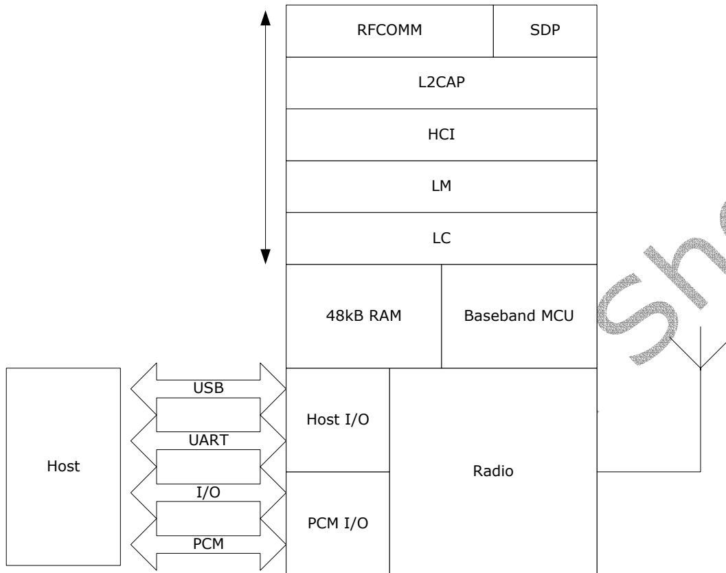
Figure 28: WRAP THOR RFCOMM stack
