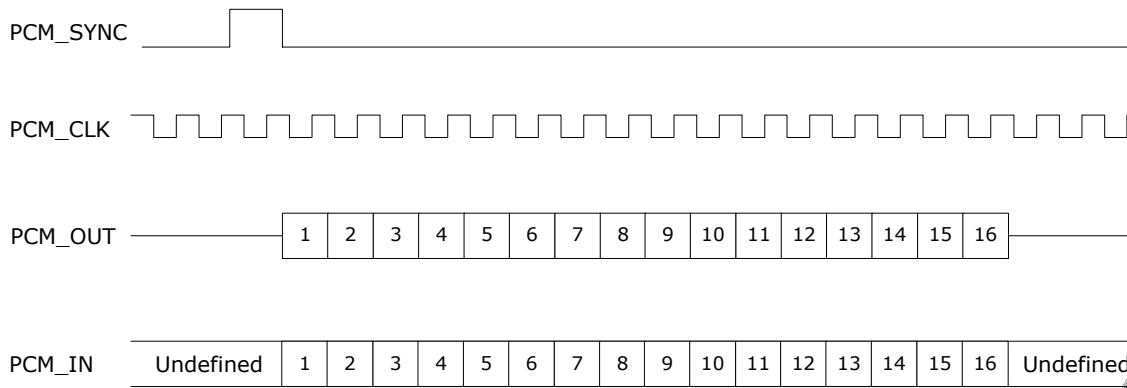
Figure 16: Short frame sync (shown with 16-bit Companded Sample)
