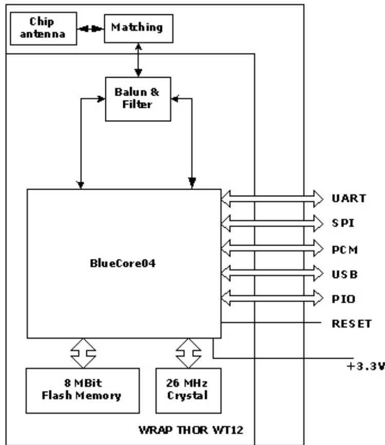
Figure 1: Block Diagram of WT12
