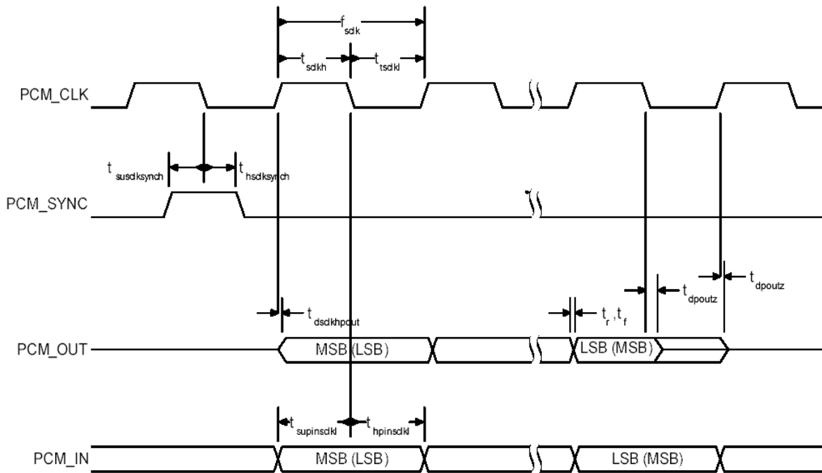
Figure 26: PCM slave timing short frame sync
