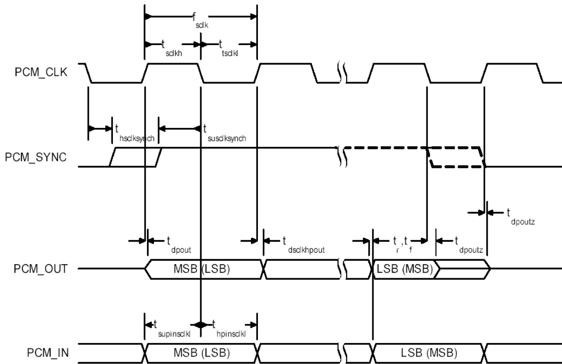
Figure 25: PCM slave timing long frame sync
