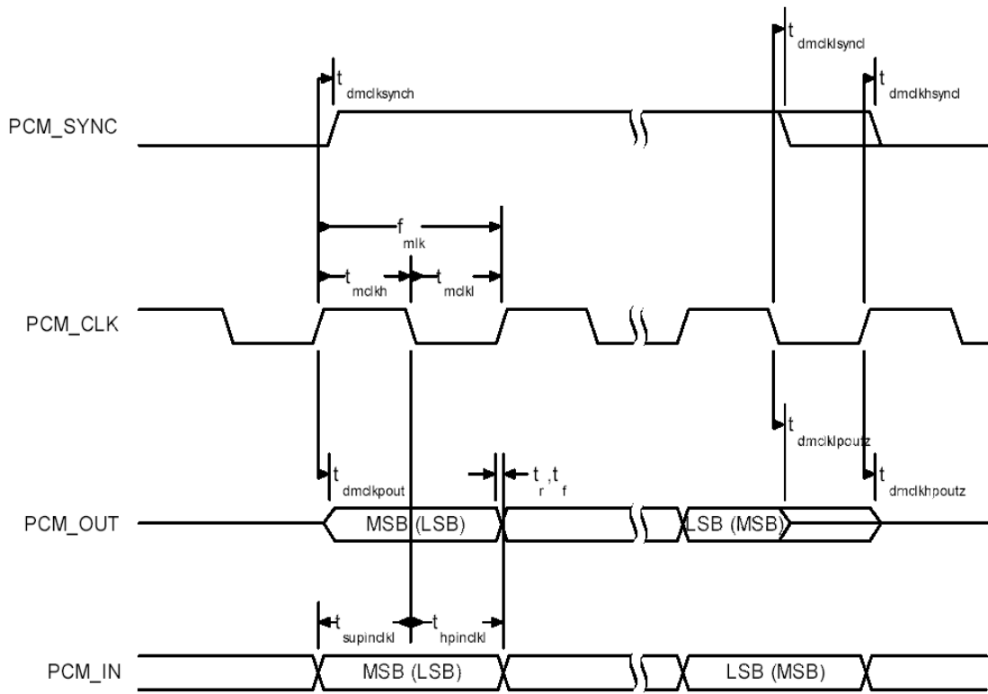
Figure 23: PCM master timing long frame sync
