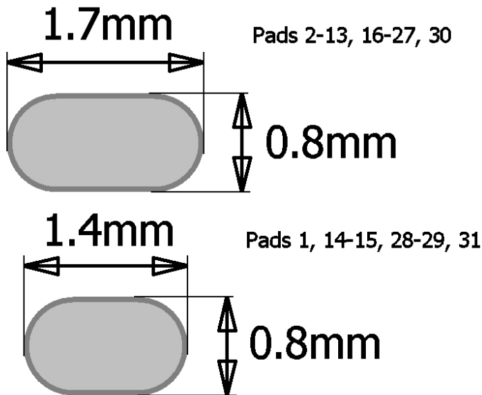
Figure 3: WT12 pad dimensions
