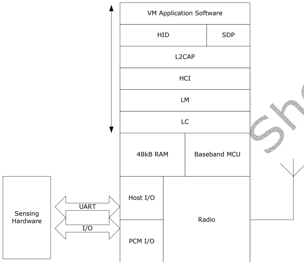
Figure 30: WRAP THOR HID stack
