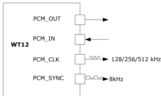
Figure 13: WT12 as PCM master
