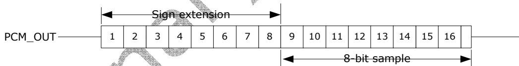
Figure 19: 16-bit slot with 8-bit companded sample and sign extension selected
