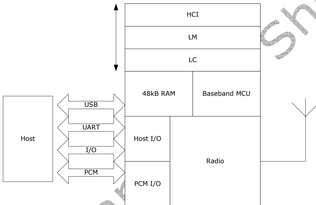
Figure 27: WRAP THOR HCI Stack
