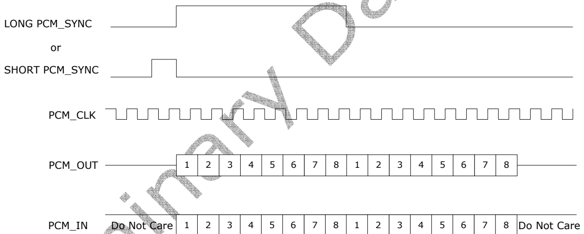
Figure 17: Multi Slot Operation with Two Slots and 8-bit Companded Samples
